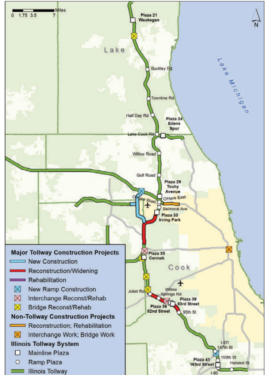
Figure 2-29 | Tri-State Tollway Construction (2021)
